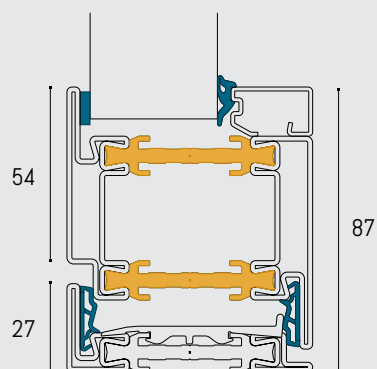
WINDOW LOWER INTERSECTION
