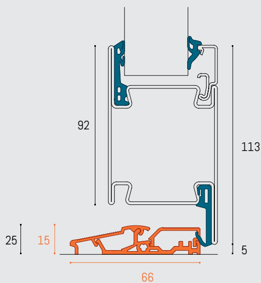
BALCONY DOOR LOWER INTERSECTION
