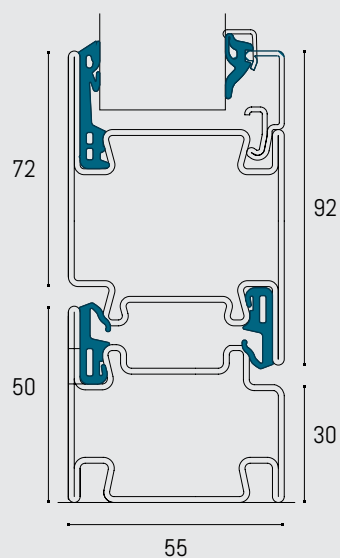
WINDOW LOWER INTERSECTION
