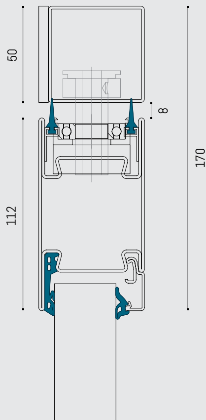
PIVOT DOOR UPPER INTERSECTION
