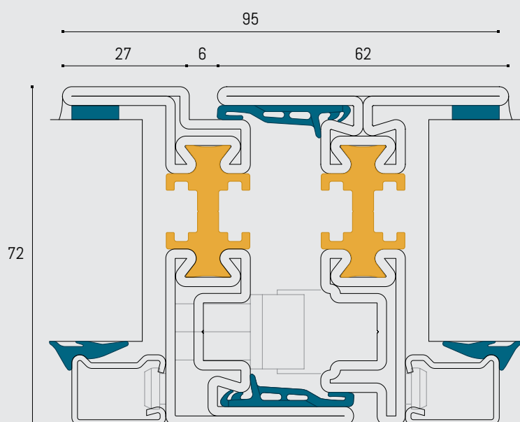
BALCONY DOOR CENTRAL INTERSECTION
